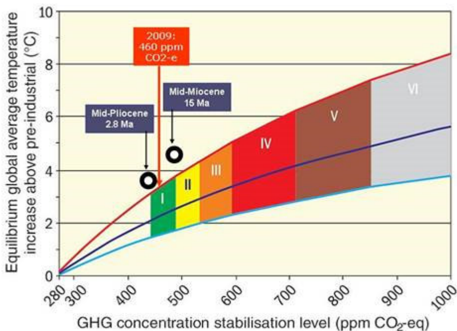
Figure 2. The relations between atmospheric CO 2 -equivalent (including the radiative forcing of methane) and mean global temperature, according to Charney's climate sensitivity parameter (Hansen et al., 2007, 2008) (IPCC-2007). Circles mark new paleoclimate estimates of atmospheric conditions in the mid-Pliocene (2.8 million years ago) and the mid-Miocene (15 million years ago), with implications to current climate trajectories.
